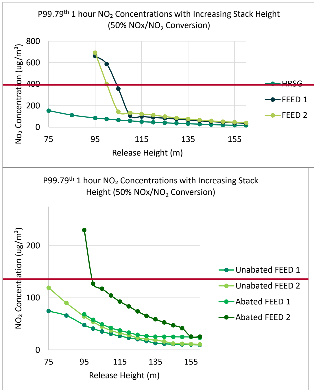
Plate 2: Predicted Maximum Process Contribution to Ground Level NO 2 Concentrations at Stack Release Heights of 75 m to 160 m
